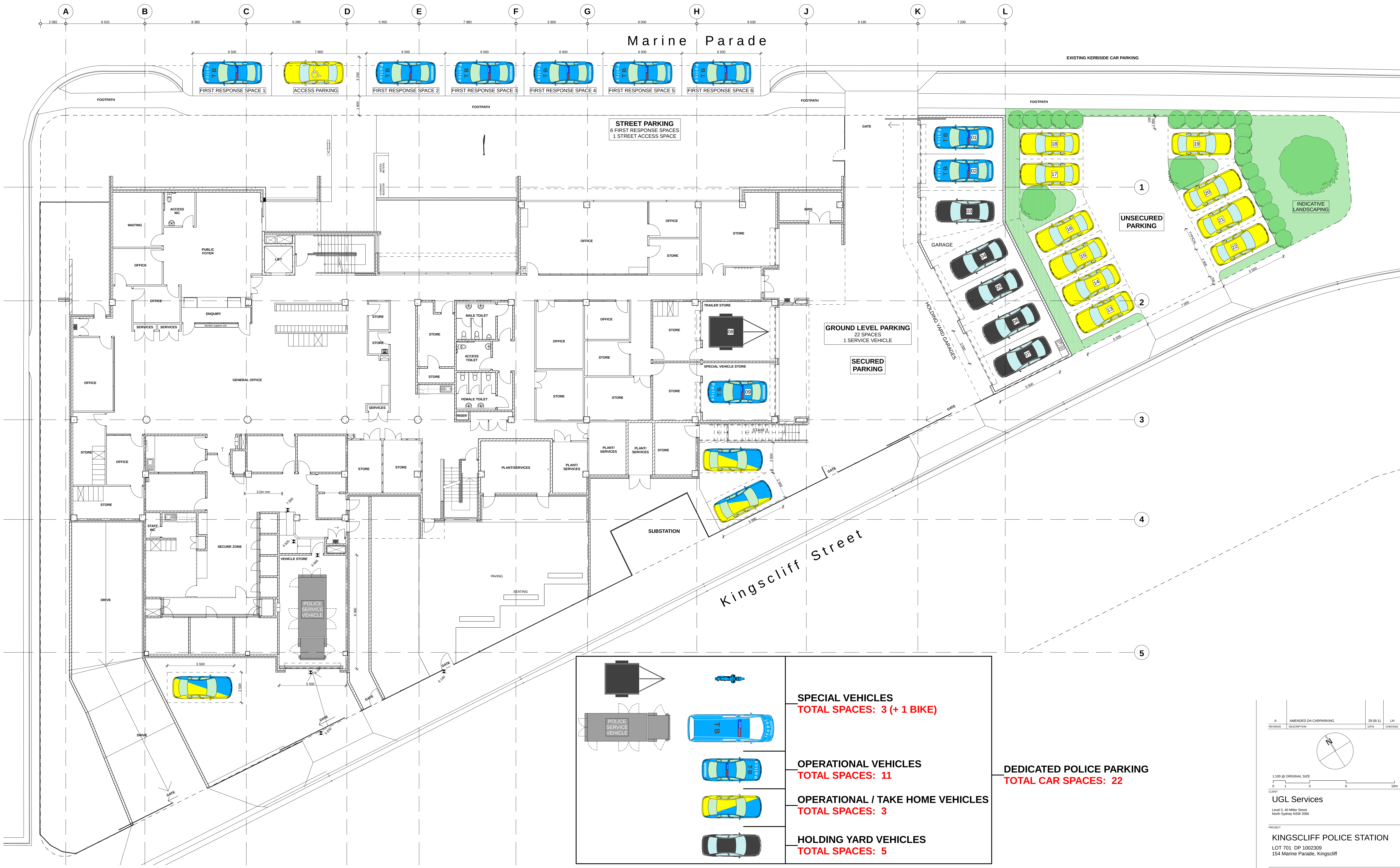
1 Vehicle Layout Plan - Ground Floor SCALE - 1:100 @ A0 SCALE - 1:200 @ A2
